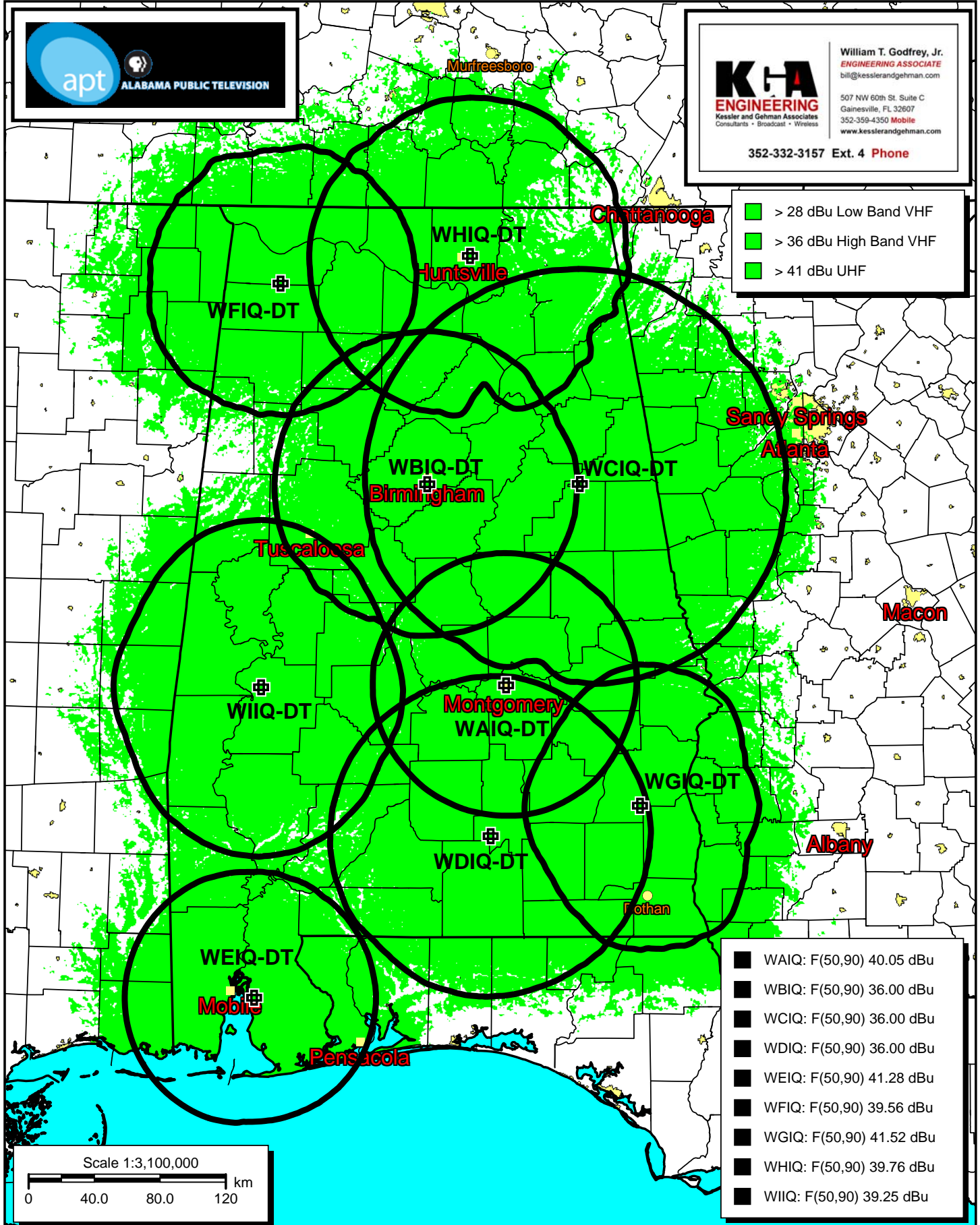
Longley-Rice Coverage Map & F(50,90) protected Contours
